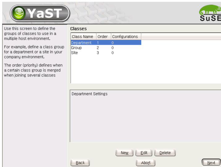
Figure 6.2 Defining Classes
