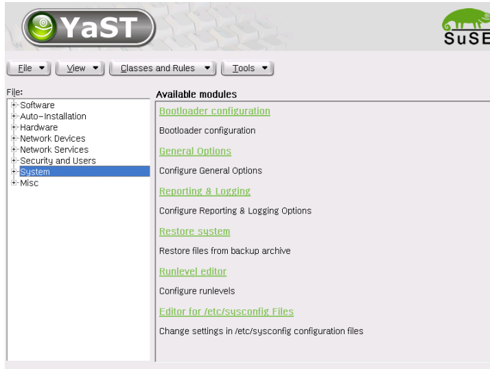
Figure 3.1 Configuration System
