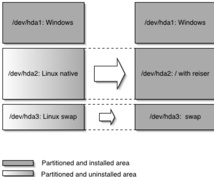
Figure 4.1 Keeping partitions
